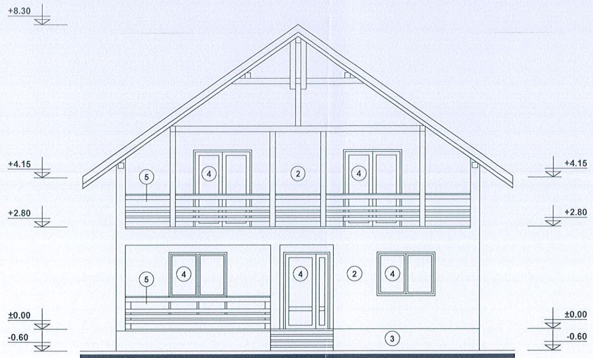
FATADA PRINCIPALA Scara 1:100
